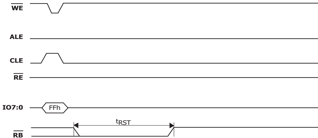
Figure 23: Reset Operation
