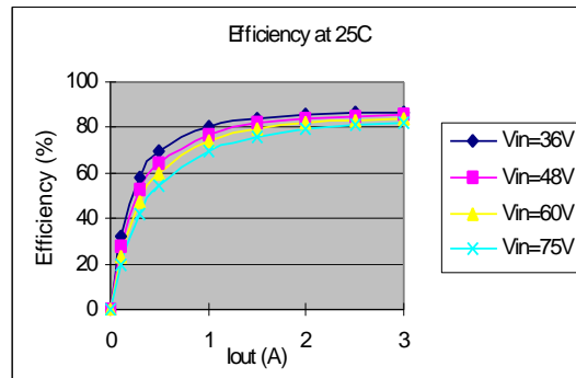
Efficiency vs. Load Current Curves for 1.8Vo
