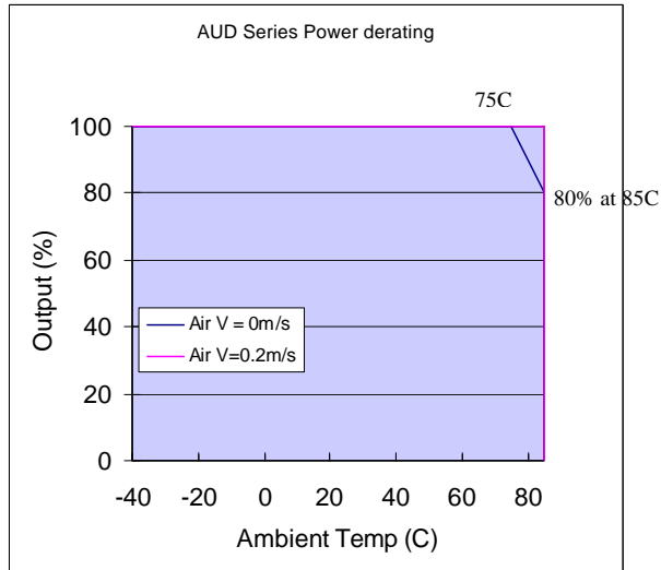
Derating Curve for the AUD Series
