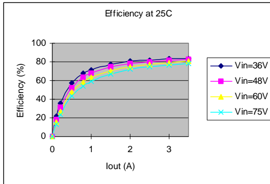
Efficiency vs. Load Current Curves for 1.5Vo
