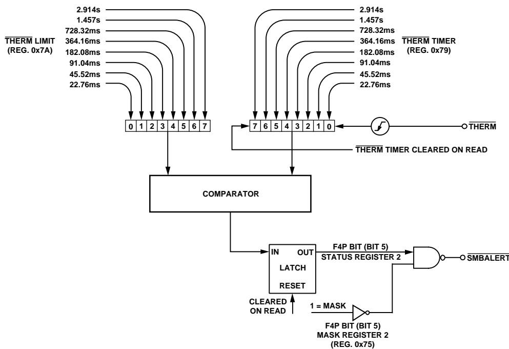
Figure 32. Functional Block Diagram of \overline{\text{THERM}} Monitoring Circuitry
