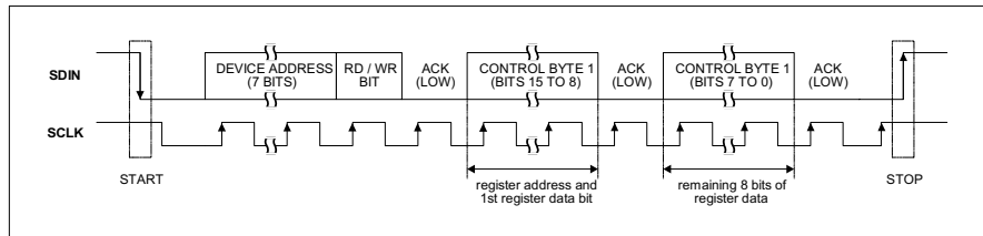
Figure 18 2-Wire Serial Control Interface
