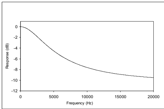
Figure 33 De-Emphasis Frequency Response (44.1kHz)
