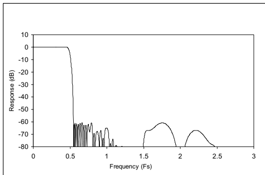
Figure 27 Digital Filter Frequency Response – 44.1, 48 and 96kHz
