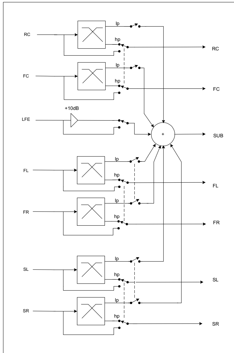
Figure 20 Bass Management
