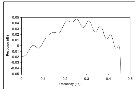
Figure 28 Digital Filter Ripple – 44.1, 48 and 96kHz
