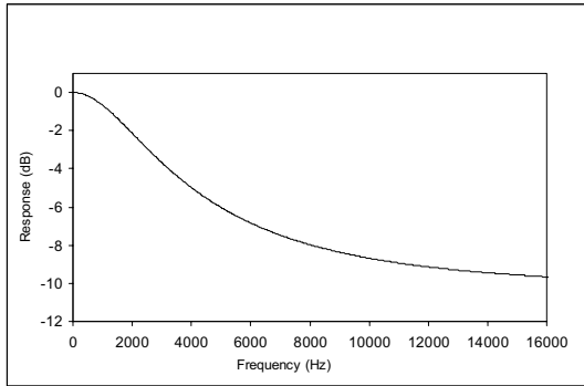
Figure 31 De-Emphasis Frequency Response (32kHz)
