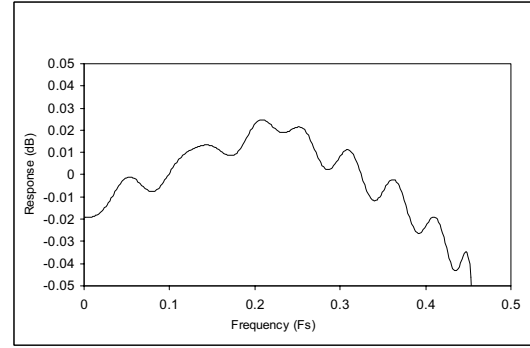
Figure 26 Digital Filter Ripple – 32kHz
