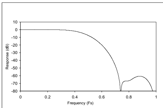
Figure 29 Digital Filter Frequency Response – 176.4kHz and 192kHz
