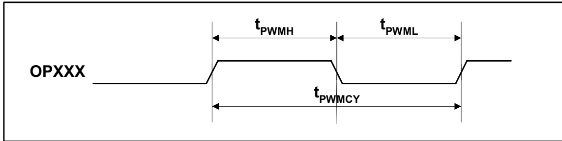
Figure 6 PWM Output Timing
