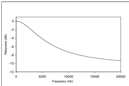
Figure 35 De-Emphasis Frequency Response (48kHz)
