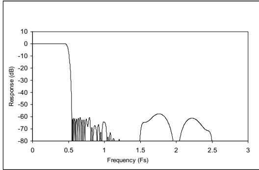
Figure 25 Digital Filter Frequency Response – 32kHz
