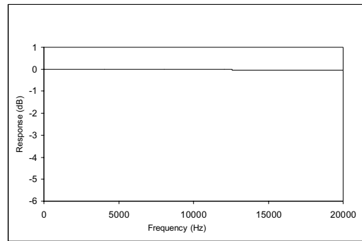
Figure 34 De-Emphasis Error (44.1kHz)
