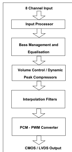
Figure 7 Signal Processing Block Diagram
