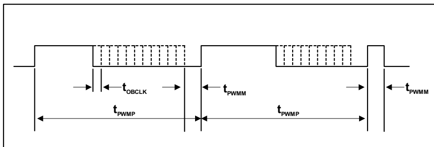
Figure 23 PCM to PWM Converter
