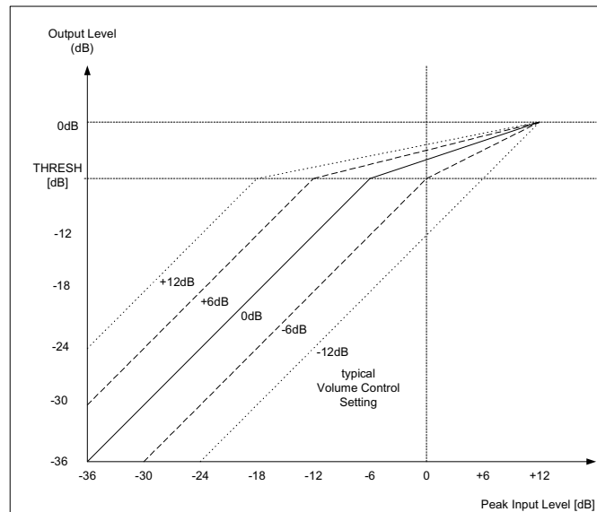
Figure 22 Dynamic Peak Compressor Characteristics
