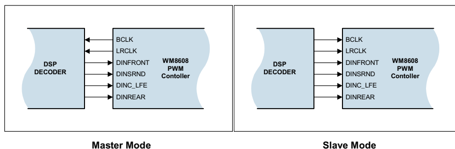
Figure 8 Operation Mode
