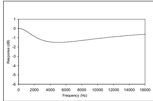
Figure 32 De-Emphasis Error (32kHz)
