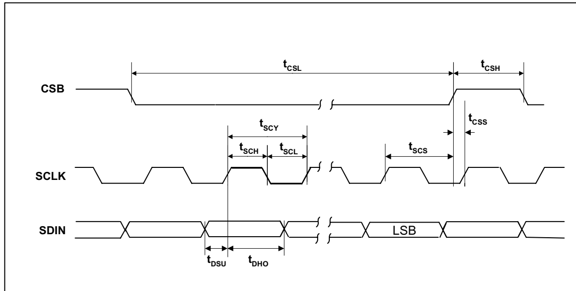
Figure 4 Control Interface Timing – 3-Wire Serial Control Mode
