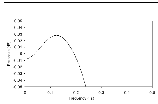
Figure 30 Digital filter Ripple – 176.4kHz and 192kHz
