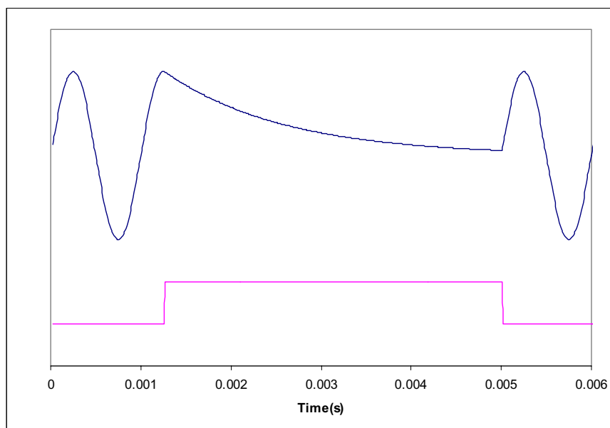
Figure 21 Application and Release of Soft Mute
