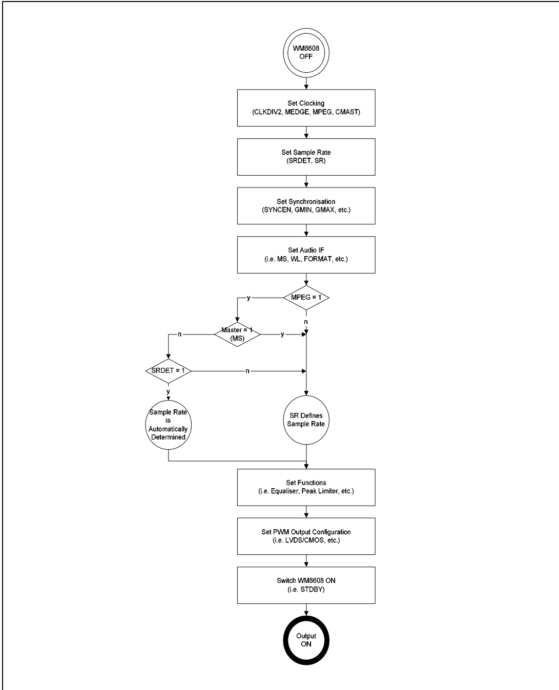
Figure 37 WM8608 Start-up
