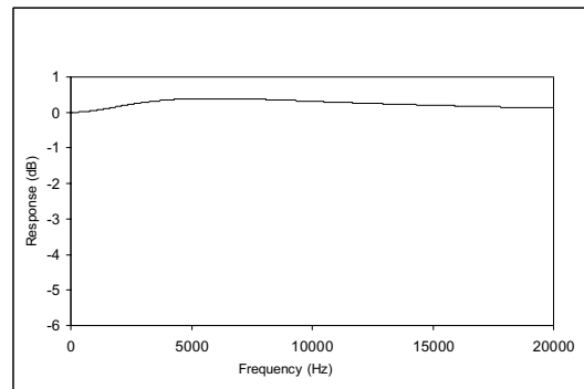
Figure 36 De-Emphasis Error (48kHz)
