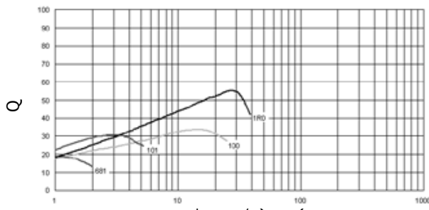
Q vs. Frequency Characteristics
