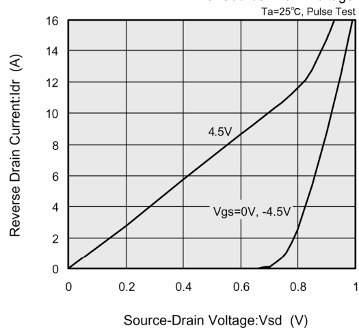
(10) Reverse Drain Current vs. Source-Drain Voltage
