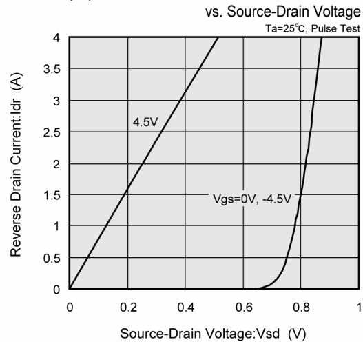
(10) Reverse Drain Current
