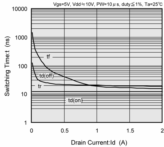
(8) Switching Time vs. Drain Current
