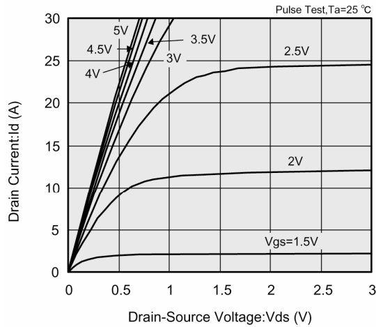
(1) Drain Current vs. Drain-Source Voltage
