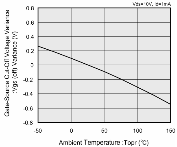
(6) Gate-Source Cut-Off Voltage Variance vs. Ambient Temperature
