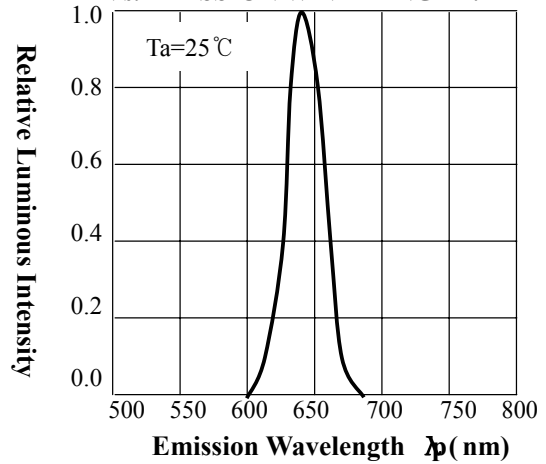
● RELATIVE LUMINOUS INTENSITY Vs. EMISSION WAVELENGTH.
