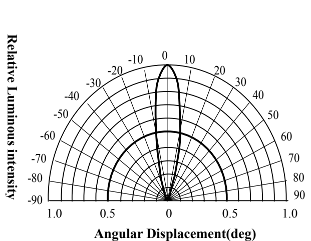
● RELATIVE LUMINOUS INTENSITY Vs. ANGULAR DIAPLACEMENT
