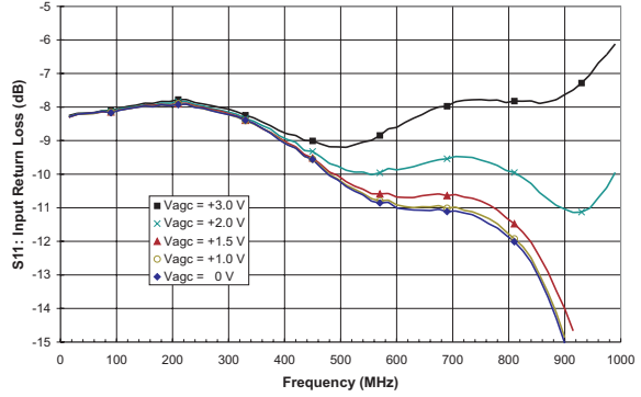
Figure 4: Input Return Loss vs. Frequency ( T_A = +25\text{ }^\circ\text{C} , V_{CC} = +5\text{ V} )
