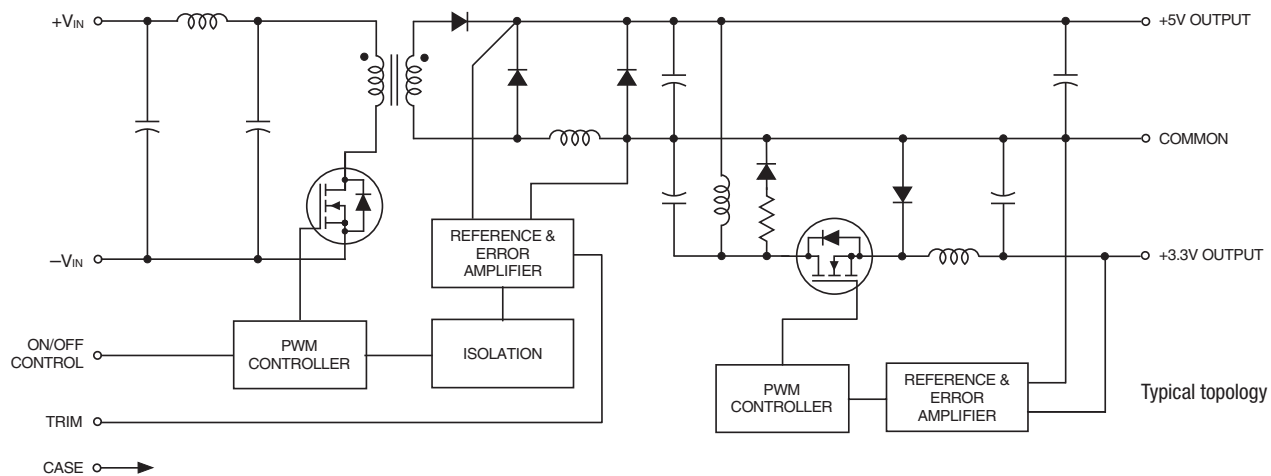
Figure 1. Simplified Schematic
