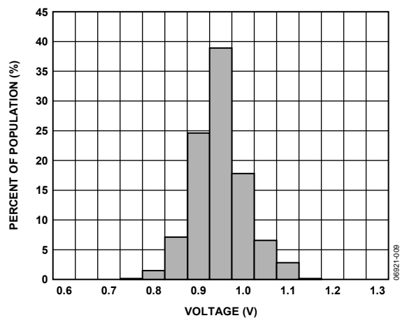
Figure 9. ST2 Output Change at 25°C ( V_{RATIO} = 5 V )
