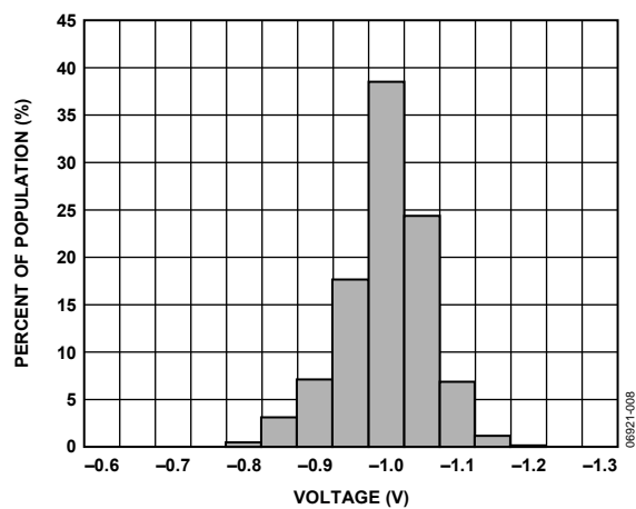
Figure 8. ST1 Output Change at 25°C ( V_{RATIO} = 5 V )
