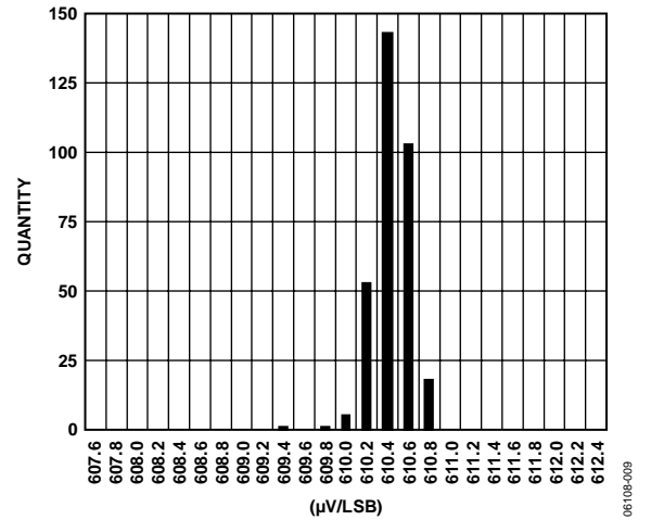
Figure 9. ADC Gain Distribution at 25°C/3.3 V
