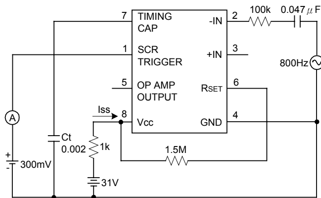
FIGURE 1. Normal Fault Sensitivity Test Circuit
