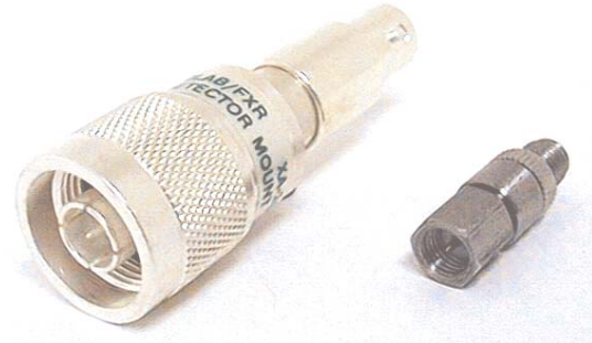
XA and miniature XF diode mounts
