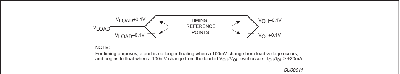
Figure 24. Float Waveform
