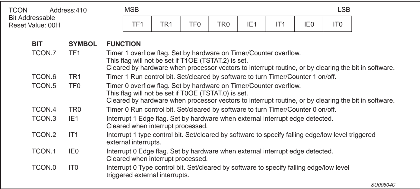
Figure 3. Timer/Counter Control (TCON) Register
