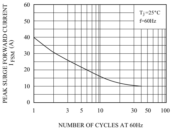
SURGE FORWARD CURRENT (NON - REPETITIVE)
