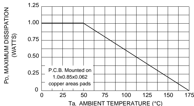
Fig. 1 MAXIMUM CONTINUOUS POWER DERATING
