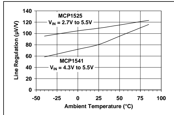
FIGURE 2-4: Line Regulation vs. Ambient Temperature.
