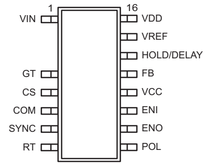
16-Lead SOIC (NG) (top view)
