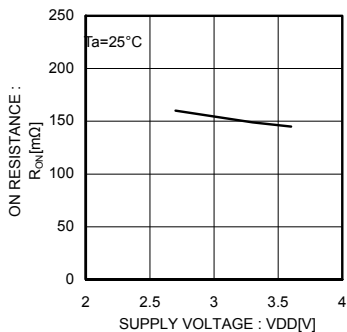
Fig.10 ON resistance
