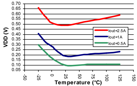
Dropout Voltage
