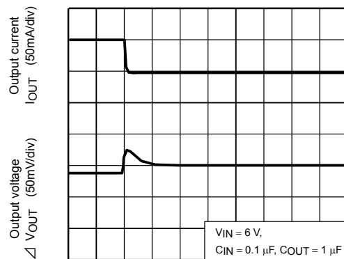
TCR5SB50U ( I_{OUT} = 100m to 50mA )
