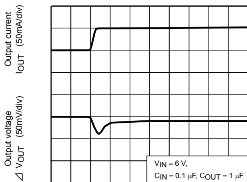
TCR5SB50U ( I_{OUT} = 50m to 100mA )
