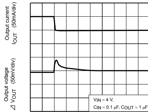
TCR5SB30U ( I_{OUT} = 100m to 50mA )
