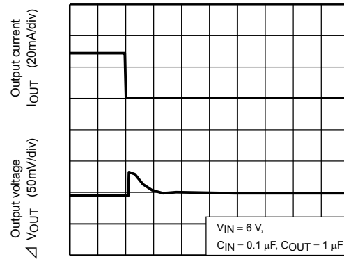
TCR5SB50U ( I_{OUT} = 30m to 1mA )
