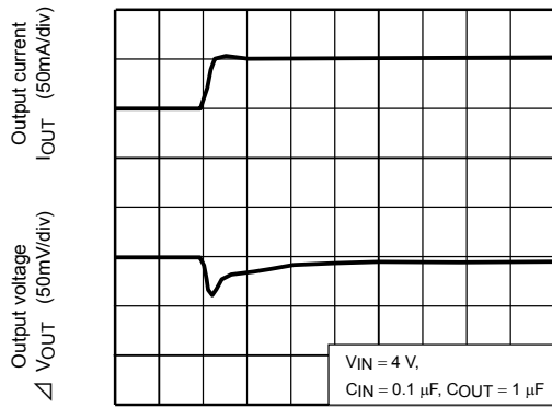
TCR5SB30U ( I_{OUT} = 50m to 100mA )
