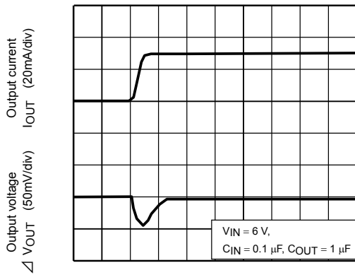
TCR5SB50U ( I_{OUT} = 1m to 30mA )
