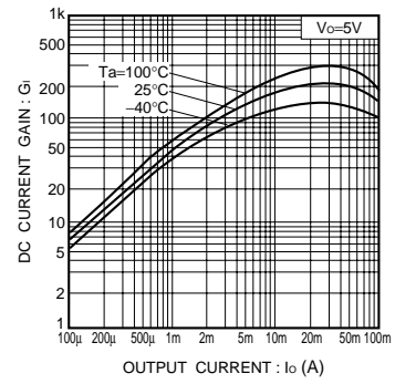
Fig.11 DC current gain vs. output current
