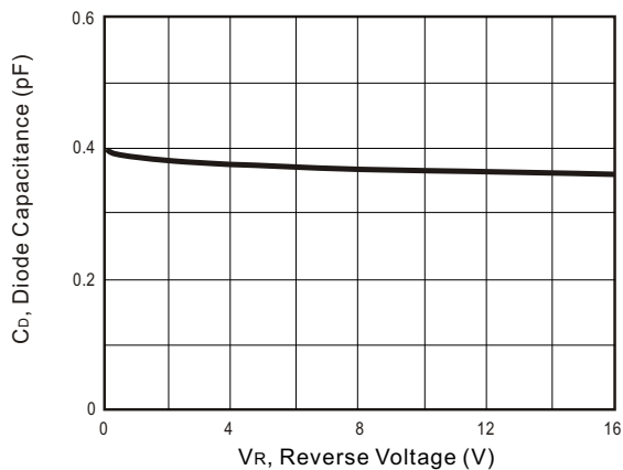
Fig.5 Diode Capacitance Characteristics
