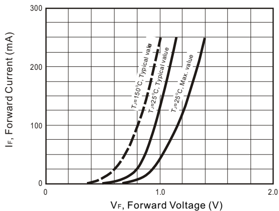
Fig.2 Forward Characteristics
