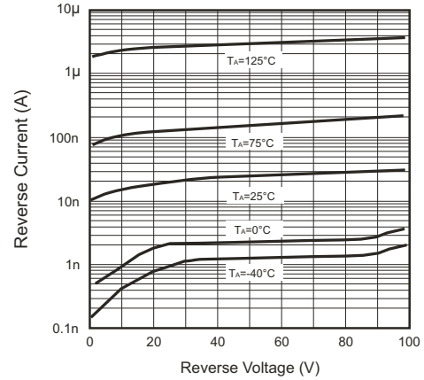
Fig.2 Reverse Characteristics
