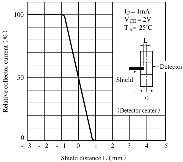
Fig.12 Relative Collector Current vs. Shield Distance (1)
