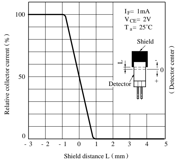
Fig.13 Relative Collector Current vs. Shield Distance (2)
