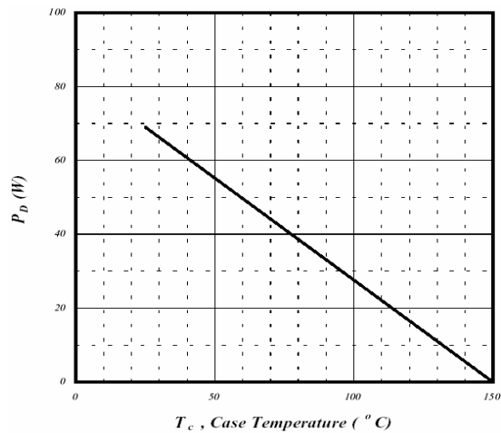
Fig. 6. Type Power Dissipation v.s. Case Temperature
