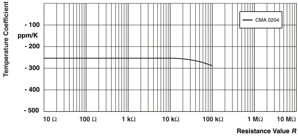
Temperature Coefficient (TCR) Temperature coefficient of resistance
