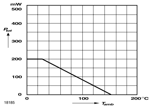
Figure 3. Admissible Power Dissipation vs. Ambient Temperature
