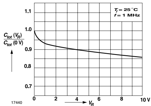
Figure 4. Relative Capacitance vs. Reverse Voltage
