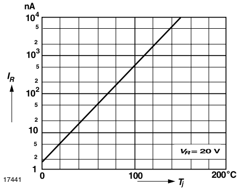
Figure 5. Leakage Current vs. Junction Temperature
