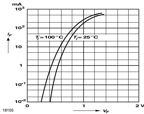
Figure 1. Forward characteristics
