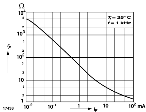
Figure 2. Dynamic Forward Resistance vs. Forward Current
