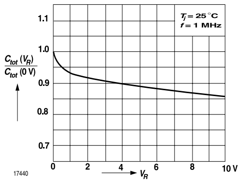
Figure 4. Relative Capacitance vs. Reverse Voltage
