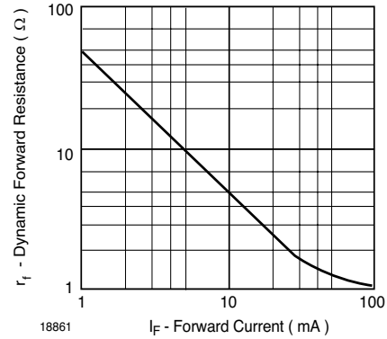
Figure 4. Dynamic Forward Resistance vs. Forward Current
