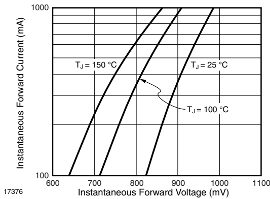
Figure 2. Typical Instantaneous Forward Characteristics
