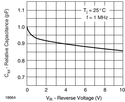
Figure 4. Relative Capacitance vs. Reverse Voltage
