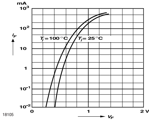
Figure 1. Forward characteristics
