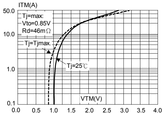
Fig.10: On-state characteristics (maximum values).
