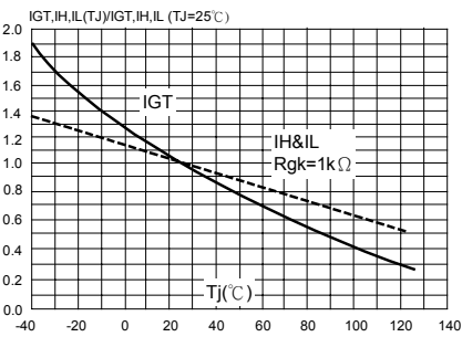
Figure.4:Relative variation of gate trigger current,holding current and latching vs junction temperature. (US108S)
