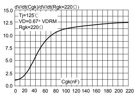
Fig.7: Relative variation of dV/dt immunity vs gate-cathode resistance (typical values) (US108S)
