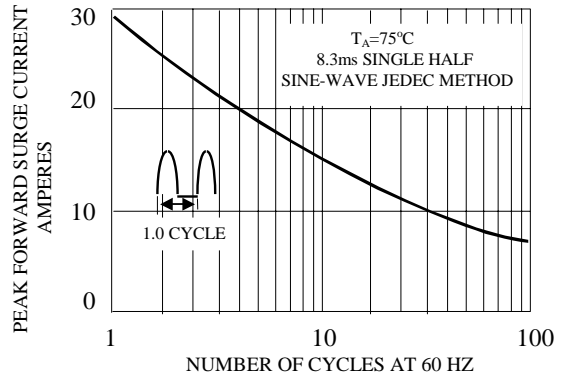
Fig. 5-MAXIMUM FORWARD SURGE CURRENT
