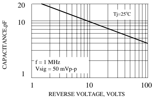
FIG. 4-TYPICAL REVERSE CHARACTERISTICS
