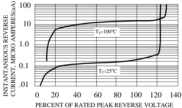
FIG. 4-TYPICAL REVERSE CHARACTERISTICS
