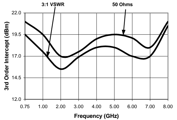
3rd Order Intercept vs. IF Port Termination 3
