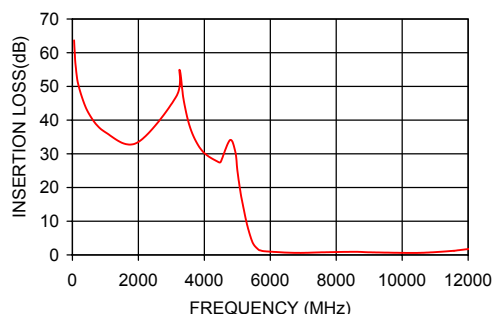
VHF-5500 INSERTION LOSS
