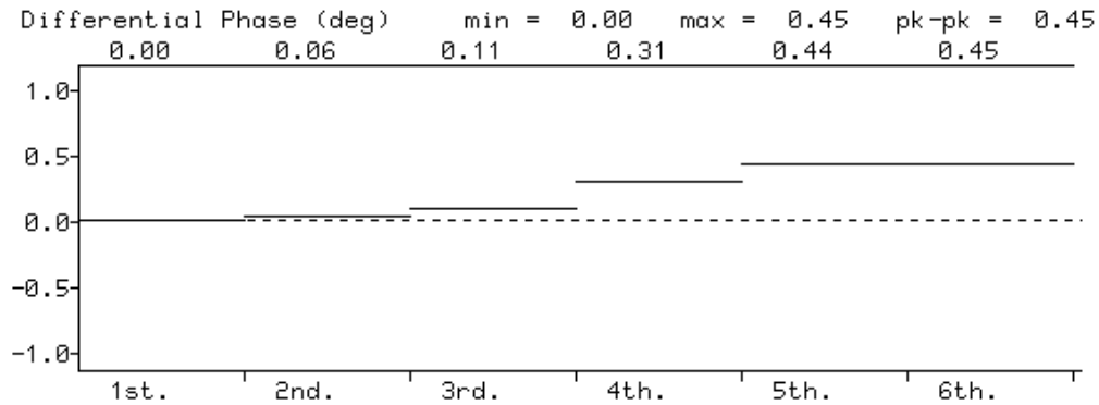
Figure 8. Differential Phase
