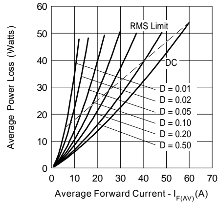
Fig. 6 - Forward Power Loss (per diode)
