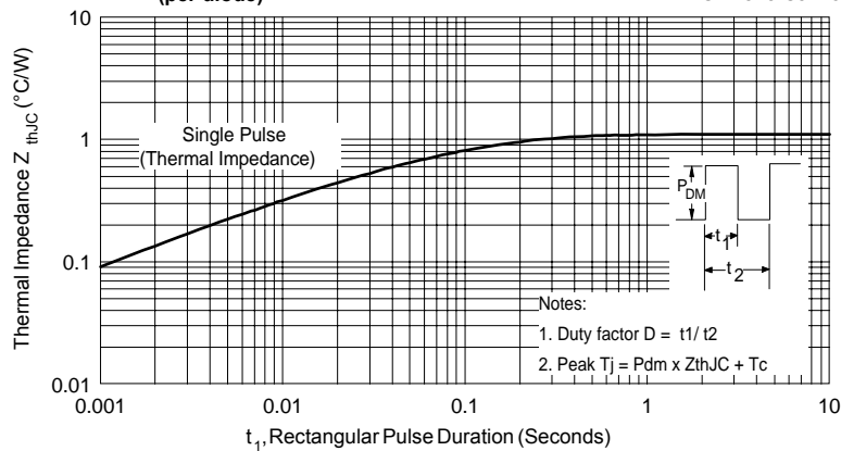
Fig. 4 - Max. Thermal Impedance Z_{thJC} (per diode)
