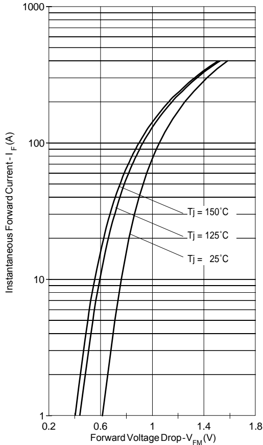
Fig. 1 - Typical Forward Voltage Drop Characteristics (per diode)
