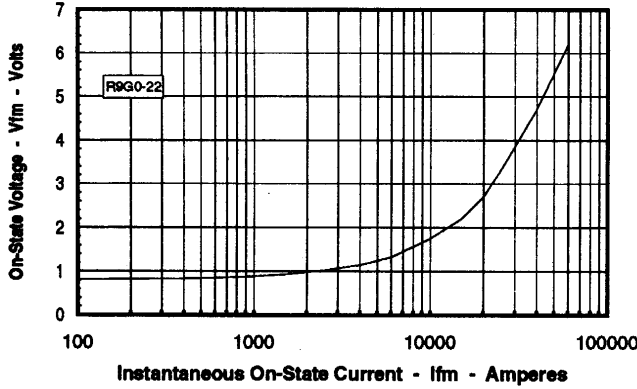
Maximum On-State Forward Voltage Drop (T j = 190 °C)
