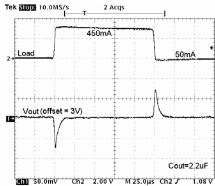
Figure 14. 10% to 90% Load Step ( t_r=1\mu s , C_{OUT}=2.2\mu F )
