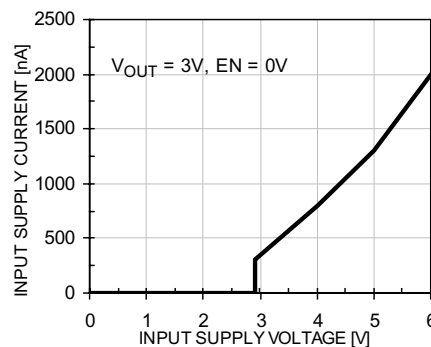
Figure 11. Input Supply Current vs. Voltage
