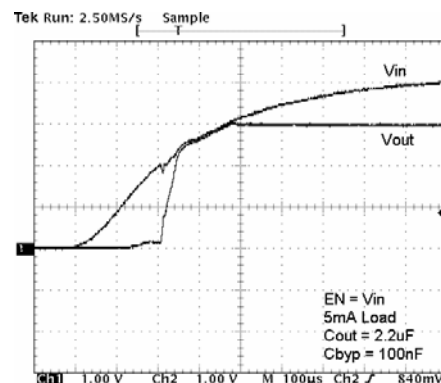
Figure 23. Power-Up ( EN=V_{IN} , I_{LOAD}=5mA , C_{OUT}=2.2\mu F , C_{BYP}=100nF )
