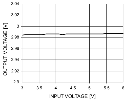
Figure 5. Line Regulation ( I_{LOAD}=5mA )
