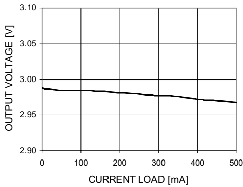
Figure 1. Load Regulation
