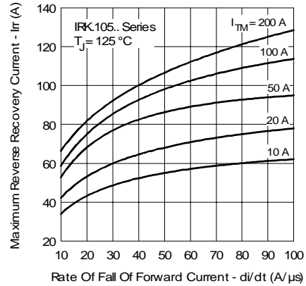
Fig. 11 - Recovery Current Characteristics
