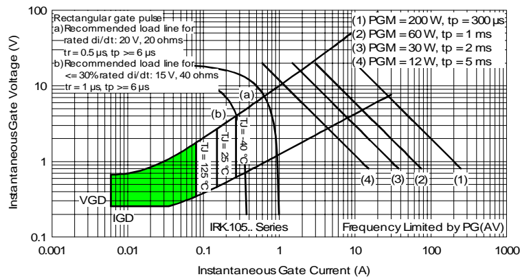
Fig. 13- Gate Characteristics
