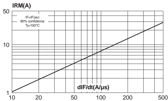
Fig. 9: Recovery current versus dI_F/dt (per diode).
