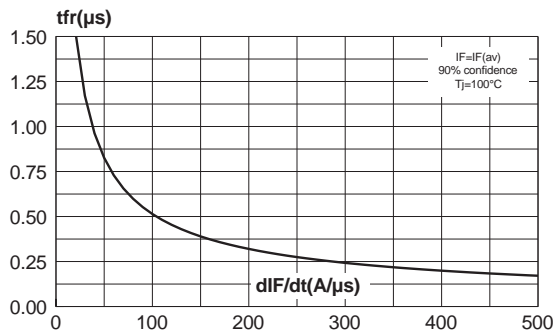
Fig. 11: Forward recovery time versus dI_F/dt (per diode).
