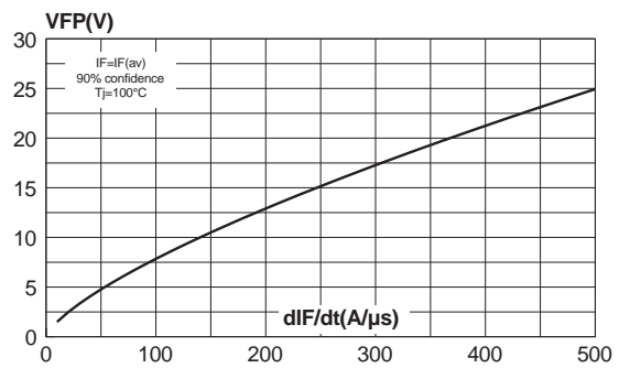
Fig. 10: Transient peak forward versus dI_F/dt (per diode).
