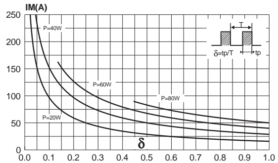
Fig. 2: Peak current versus form factor (per diode).
