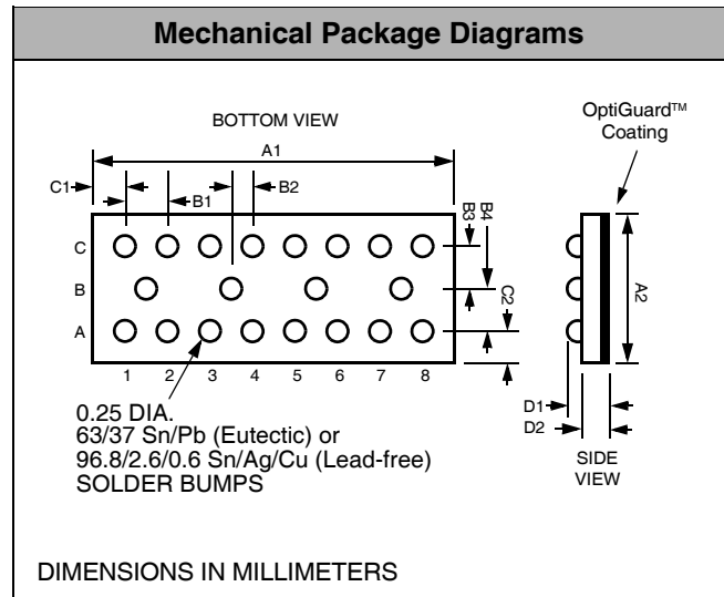
Package Dimensions for CM1442-08 Chip Scale Package
